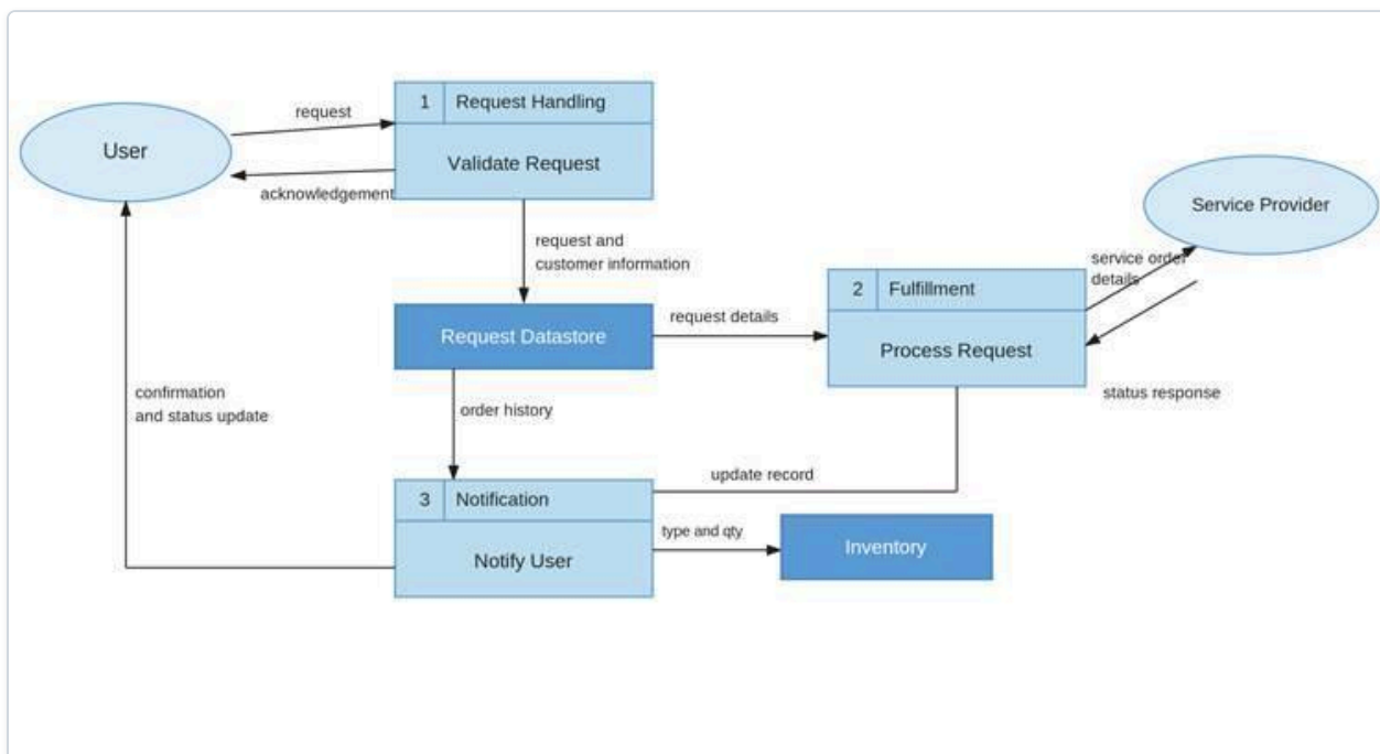
Figure 2.1: End-to-End Data Flow Diagram for Laptop Order Fulfillment
